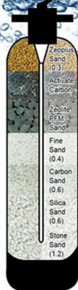
7 STEP SAND MATERIAL UPGRADE 原料提升
